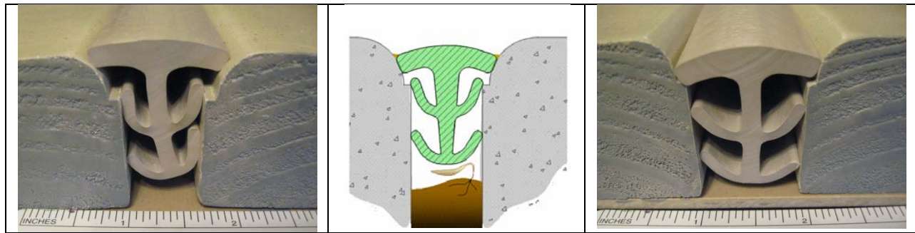
Installed in a 5/8" wide joint
